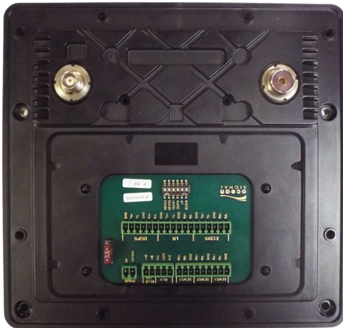
Figure 3: ATA100 – Rear View with Cover Removed
