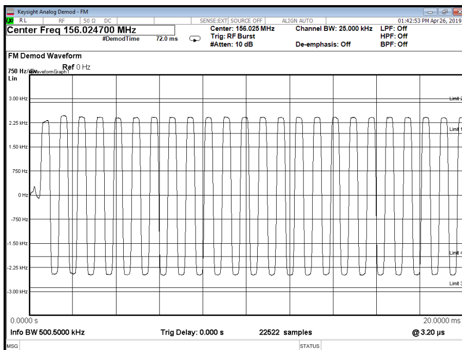
Figure 17 - 156.025 MHz, Test Signal #3, +55.0 ^{\circ} C, 31.2 V DC
