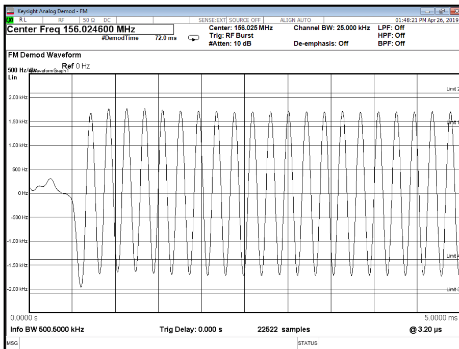
Figure 16 - 156.025 MHz, Test Signal #2, +55.0 ^{\circ} C, 31.2 V DC
