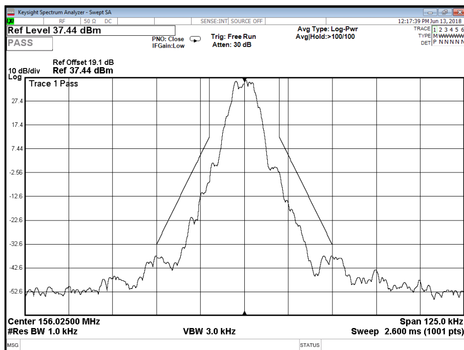
Figure 1 - 156.025 MHz
