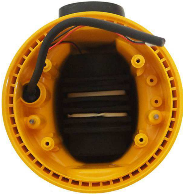
Figure 3: E101V EPIRB – Top view, case with battery assembly fitted in base.
