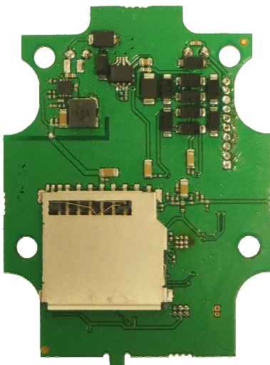
Figure 6: E101V EPIRB – VDR memory capsule PCB
