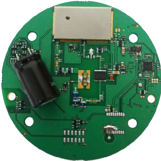
Figure 4: E101V EPIRB PCB – Component side
