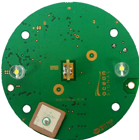
Figure 5: E101V EPIRB PCB – Top side
