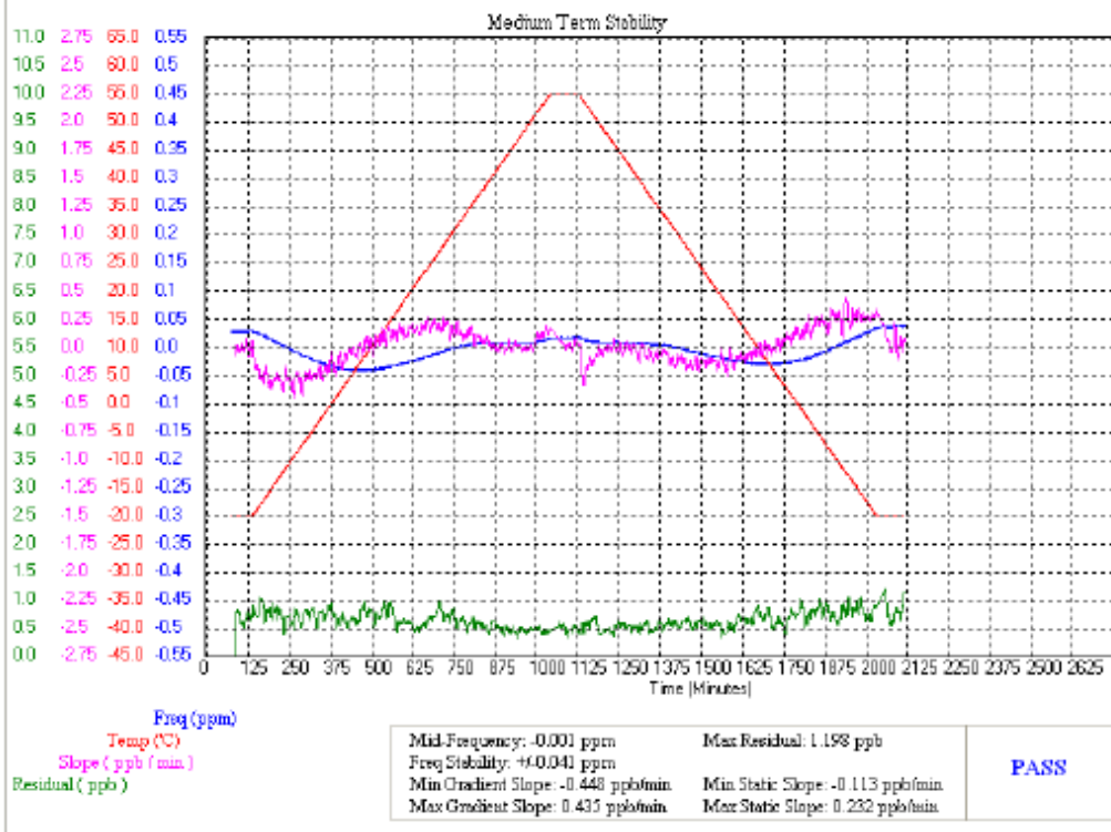
Figure 4: Frequency stability plot for crystal used in SafeSea E101V – Unit SNo 0800003P Rakon Serial N°OD6516
