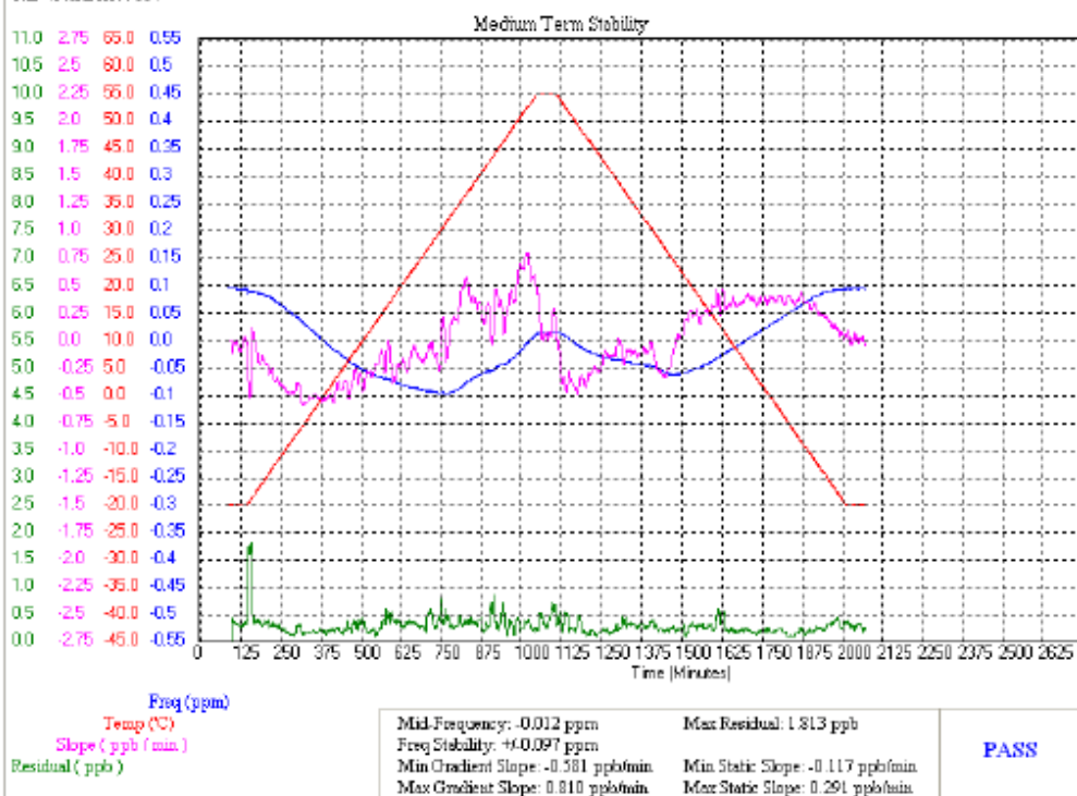
Figure 5: Frequency stability plot for crystal used in SafeSea E101V – Unit SNo 0800004P Rakon Serial N°NZ9664
