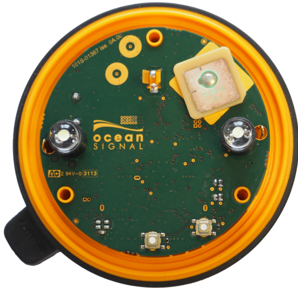
Figure 1: RescueMe EPIRB1 – Top view showing PCB in situ.
