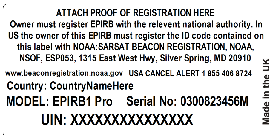
Figure 2: EPIRB1 Pro USCG information label
