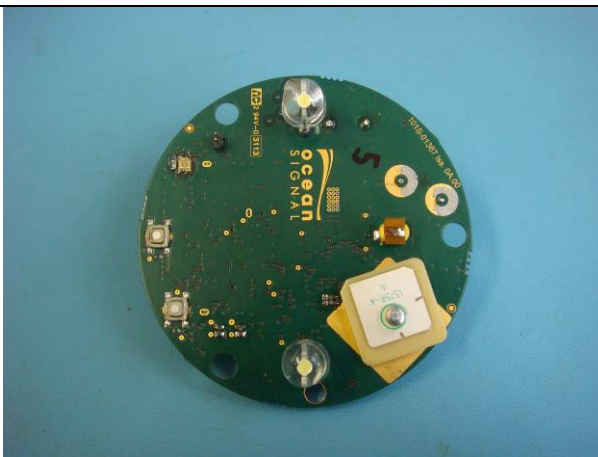
Figure 9.2 – The PCB (back view) after leakage and immersion tests. There is no water ingress.
