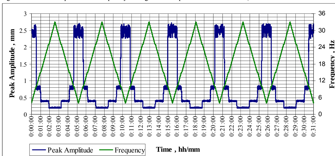
Figure 5.9 - Peak Amplitude vs. time during vibration on horizontal axis X (EPIRB1 with Manual Bracket)
