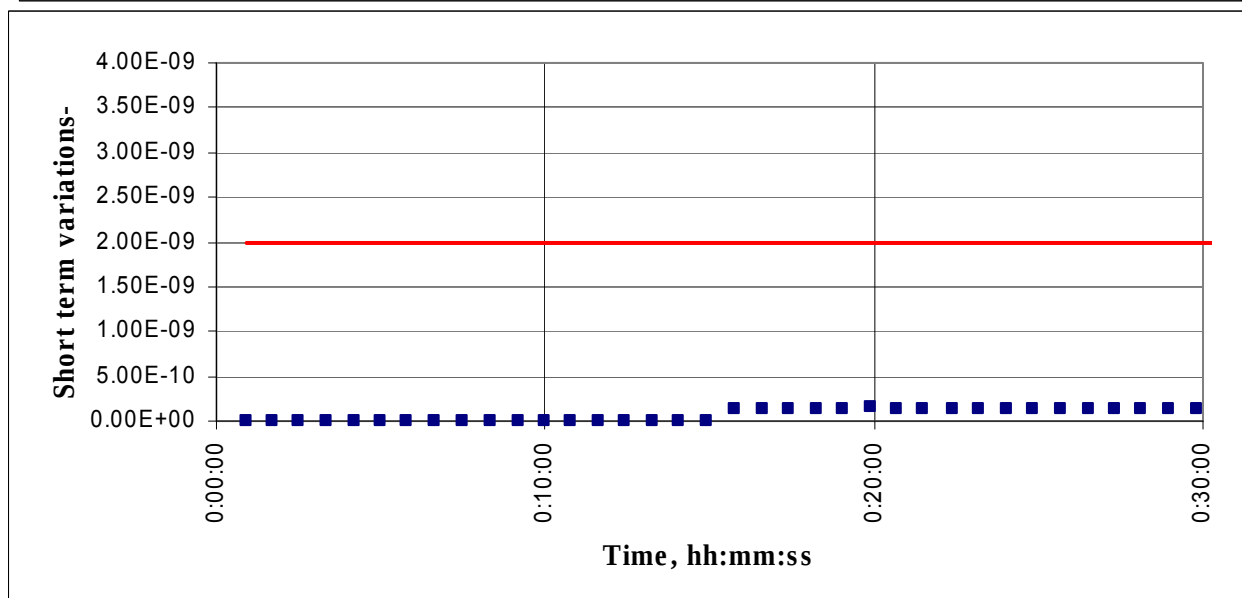
Figure 12.7 – Short-Term Stability
