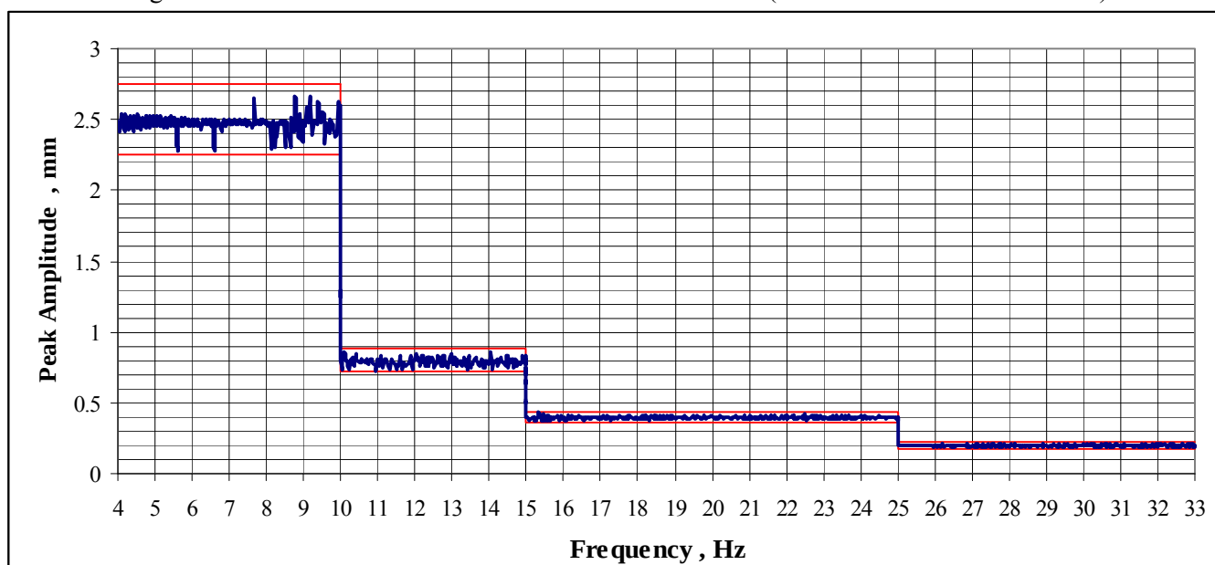
Figure 5.8 - Peak Amplitude vs. frequency during first sweep on horizontal axis X (EPIRB1 with Manual Bracket)
