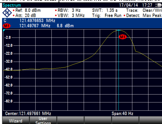
Figure 13.6 – Screenshot of Frequency Coherence Measurement Test Result (Frequency Shift) at the minimum operating temperature. Transmitted RF (121.5 MHz) before the interruption for the 406 MHz RF burst
