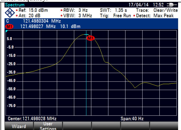
Figure 13.19 – Screenshot of Frequency Coherence Measurement Test Result (Frequency Shift) at the maximum operating temperature. Transmitted RF (121.5 MHz) after the interruption for the 406 MHz RF burst
