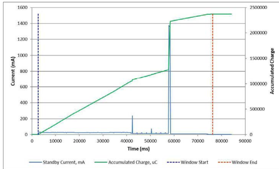
Worst Case GNSS Self-test (Burst): A10
