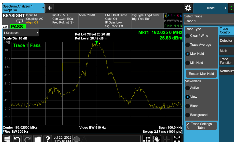
Figure 6 – 162.025 MHz - Transmitter Spectrum Mask
