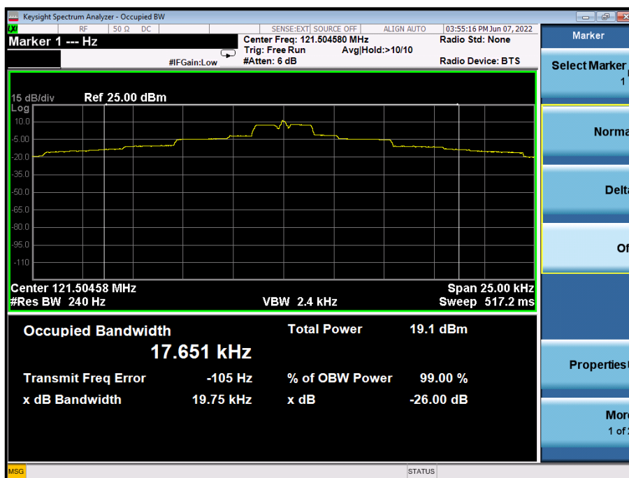
Figure 27 - Occupied Bandwidth
