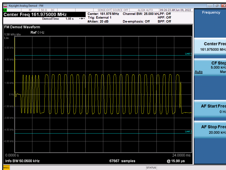
Figure 22- 161.975 MHz - 00001111
