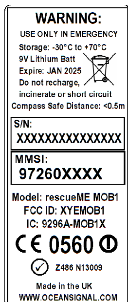
Figure 1: MOB1 Approvals Label showing FCC ID
