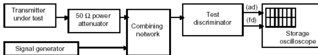
Figure A.7 – Test setup
