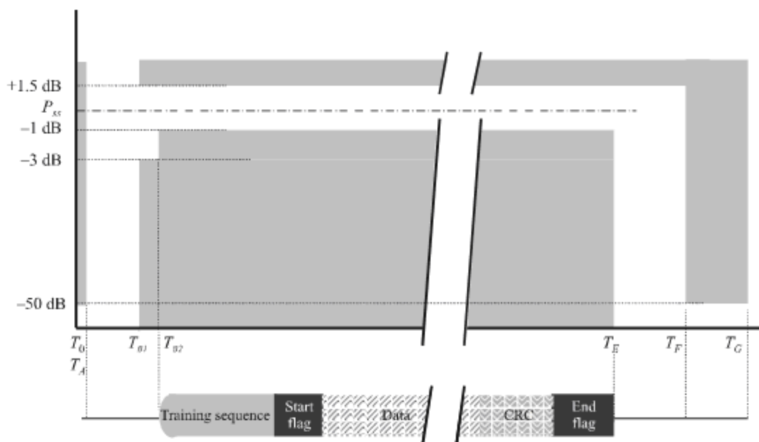
Figure E.5 – Power versus time mask
