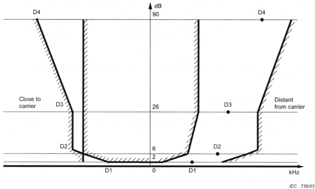
Figure A.8 – IF filter specification
