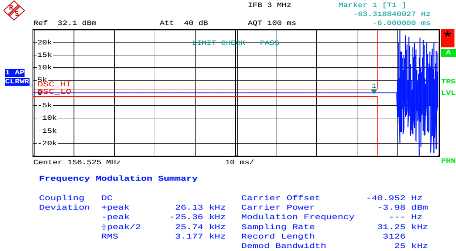
Plot 1: Transmitter transient behaviour "turn on" under normal conditions
