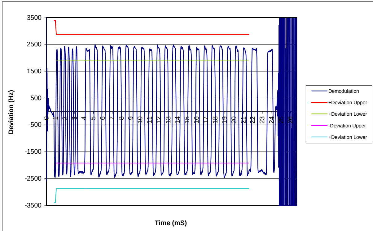
Plot 23: Transmitter transient behaviour (frequency deviation) at AIS1 frequency, test signal No.2, Upper Extreme, 55 deg C, 3.8V
