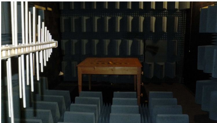
Figure 2: View of Anechoic chamber from antenna end (Used for emission prescans and immunity)
