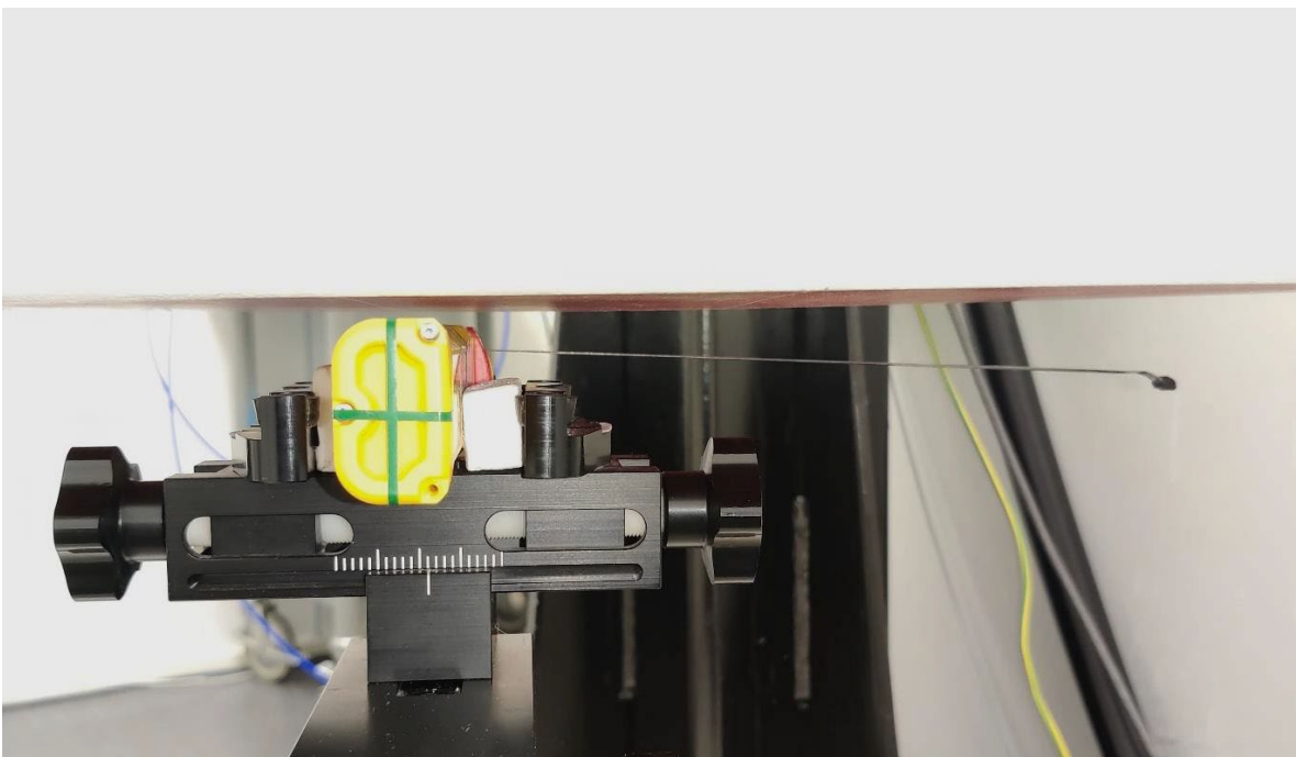
Figure 5 DUT in Antenna Left Test position
