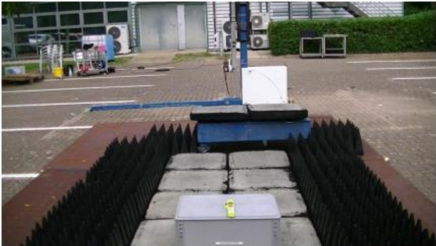
Figure 3 – Antenna Characteristics Configuration 4
