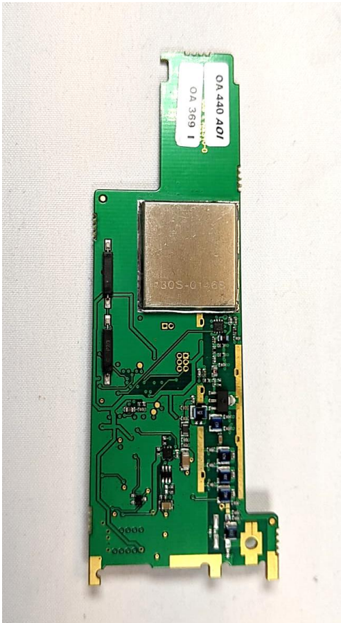
AIS SART PCB Front View
