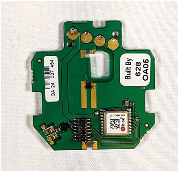
AIS SART Power PCB Front View
