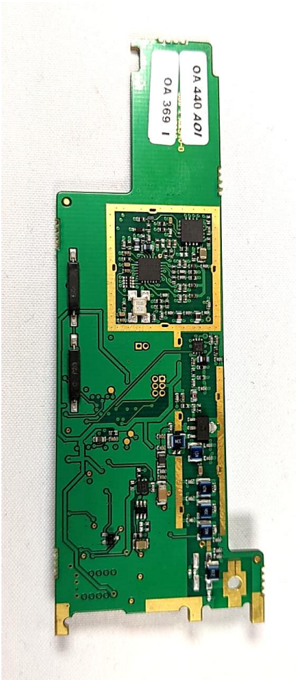
AIS SART PCB Front View with screening can removed
