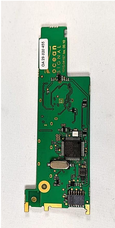
AIS SART PCB Rear View
