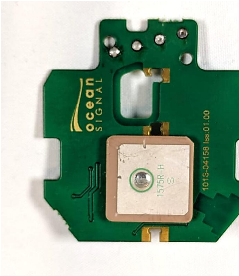
AIS SART Power PCB Rear View
