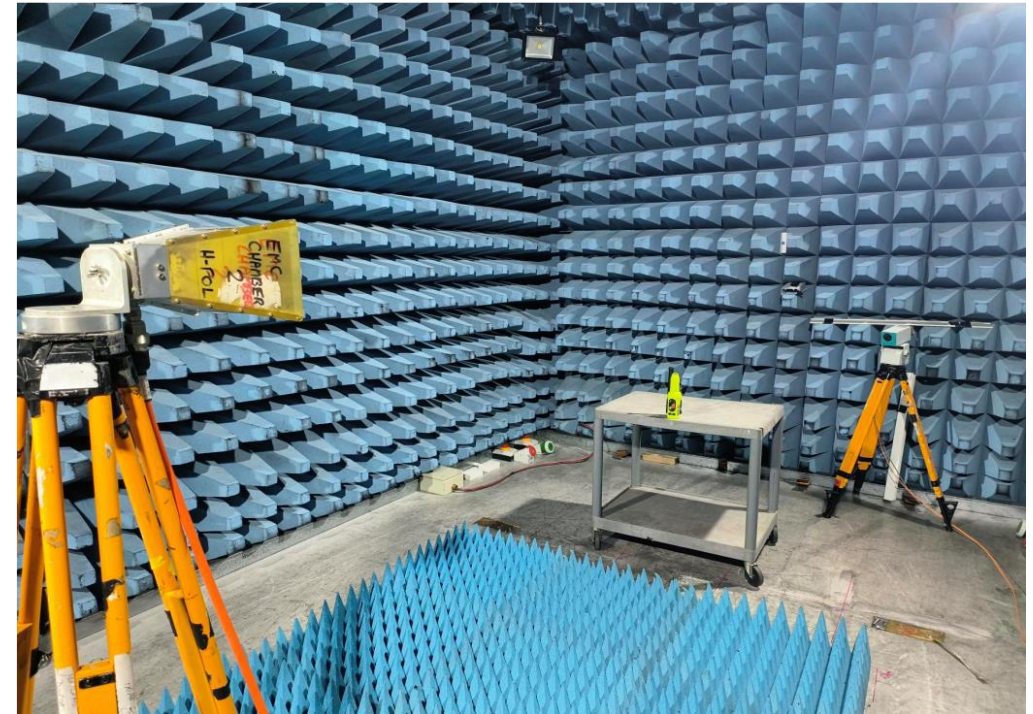
Test Setup - Above 1 GHz
