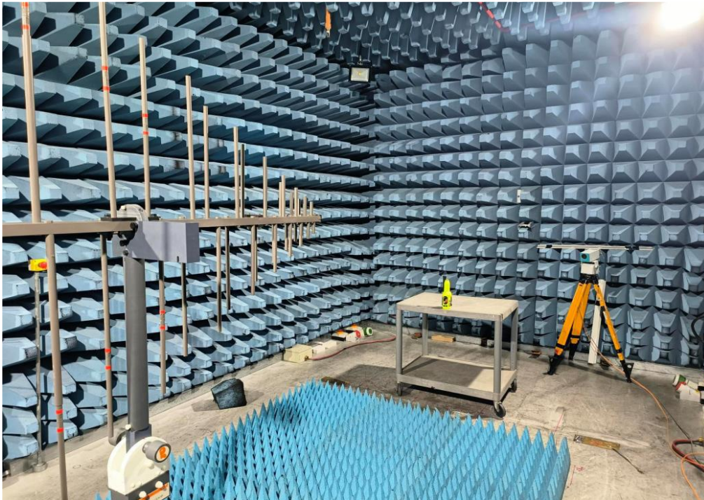
Test Setup - Below 1 GHz
