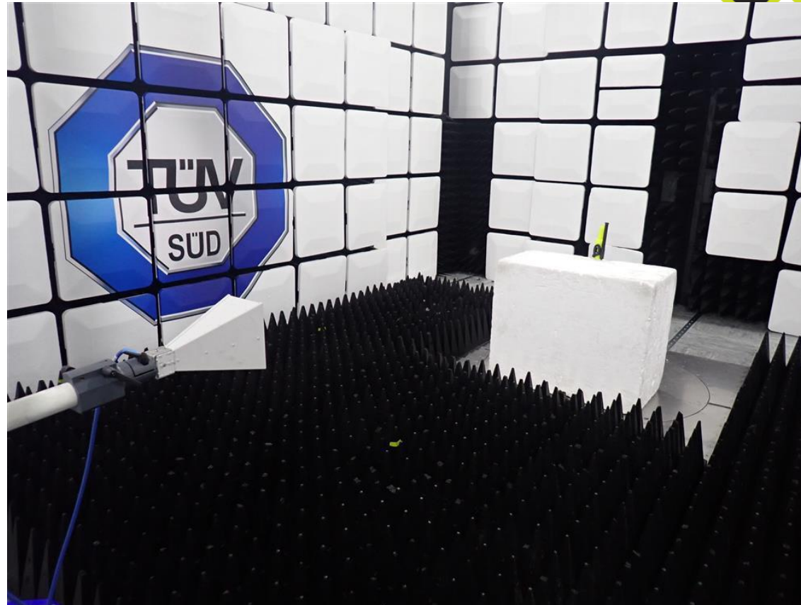
Test Setup - Above 1 GHz
