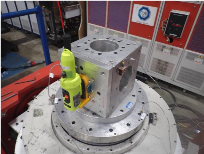
Z Axis Test Setup
