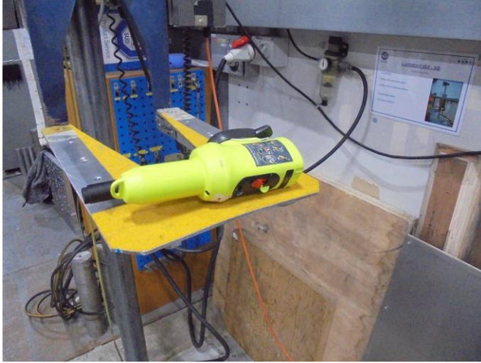
Test Setup - Drop 5
