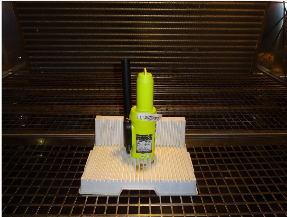
Dry Heat Test Setup – EUT in Chamber
