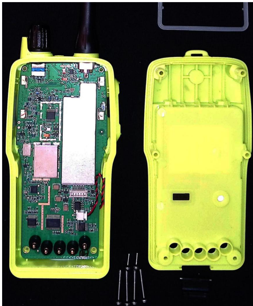
Figure 1: SR 303 VHF Internal view showing PCB in-situ
