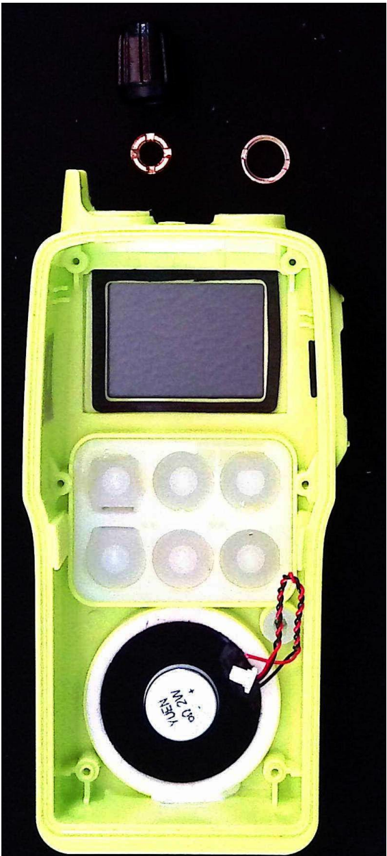
Figure 2: SR 303 VHF Internal View with PCB removed
