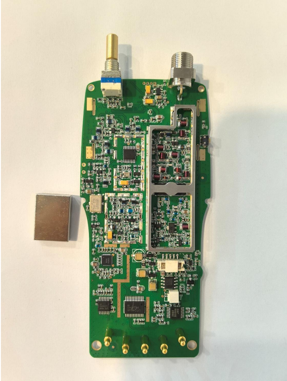
Figure 4: SR 303 VHF PCB – Rear Side with screening cans removed
