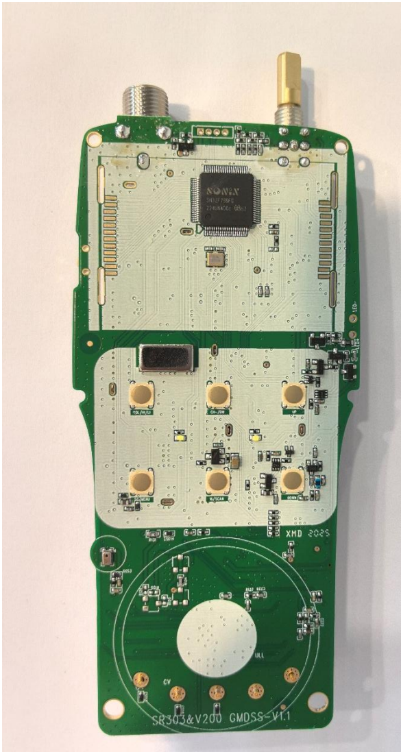
Figure 3: SR 303 VHF PCB – Front Side
