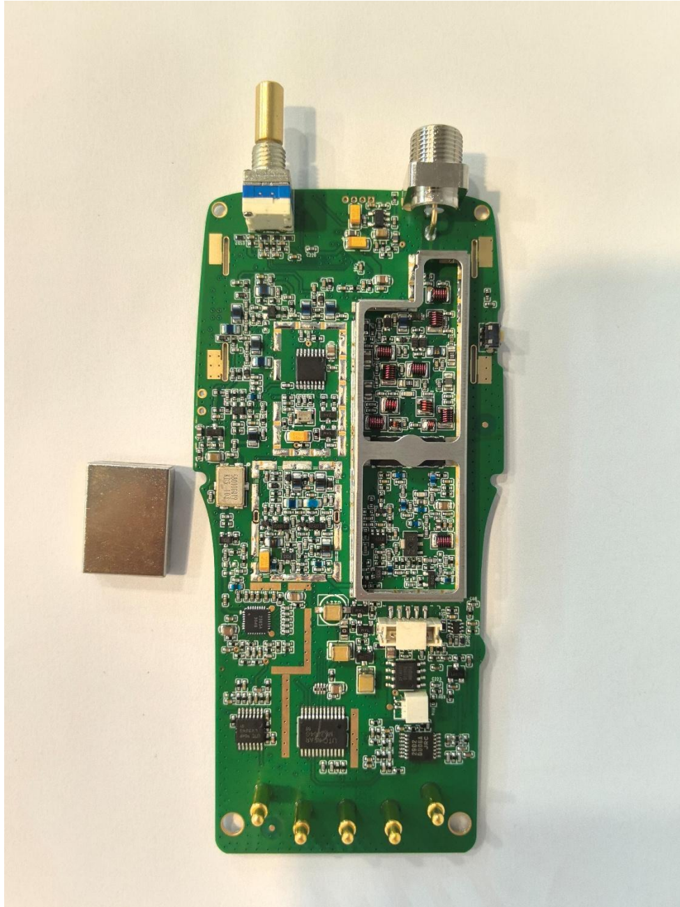
Figure 4: safeSEA V200 PCB – Rear Side with screening cans removed
