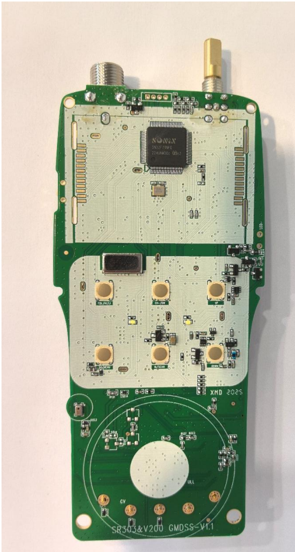
Figure 3: safeSEA V200 PCB – Front Side
