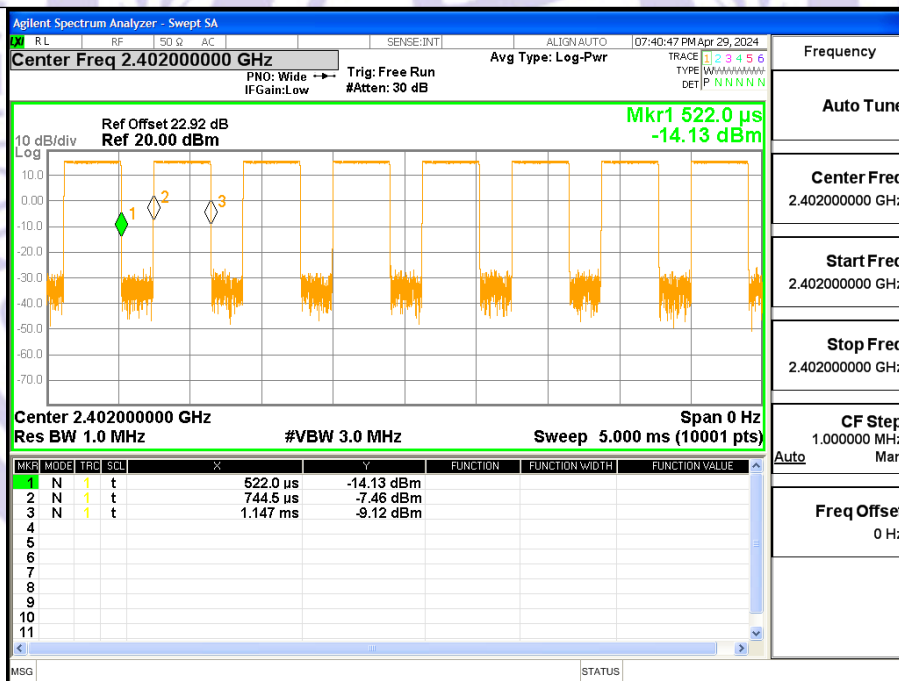
Duty_Cycle_NVNT_ANT1_1Mbps_2402
