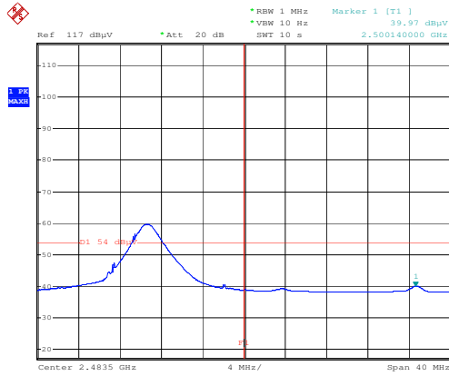
2-FSK -Left Side-PK-V
