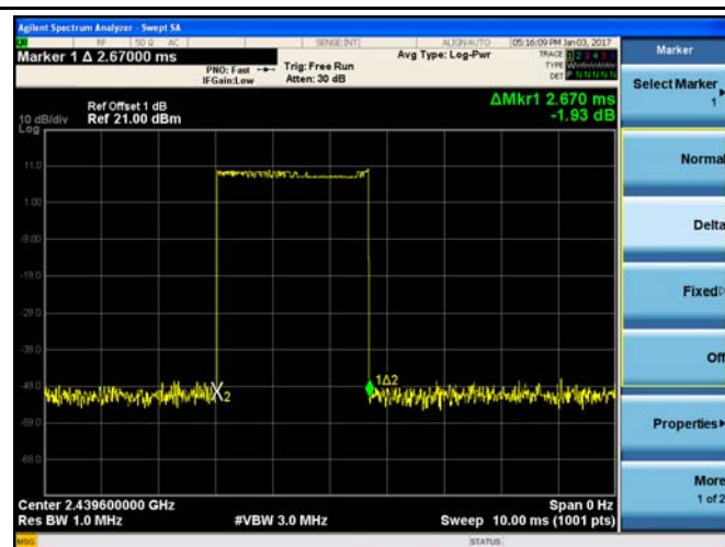
2-FSK - Mid CH 2440-ANT2#
