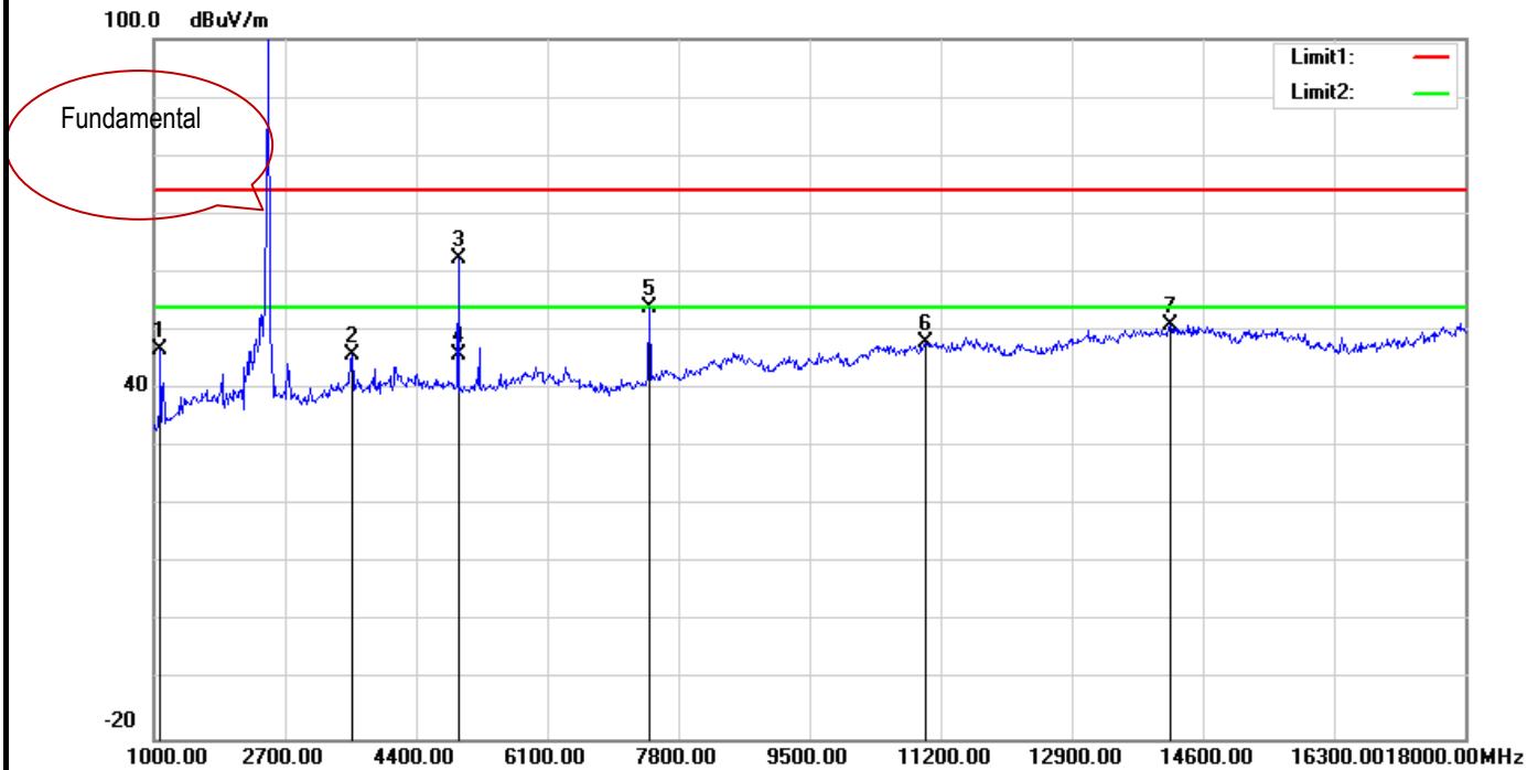
Horizontal Polarity Plot @3m
