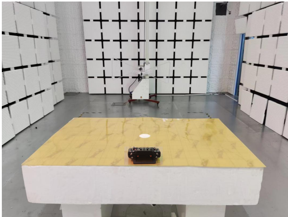
Radiation Emission 30MHz-1000MHz
