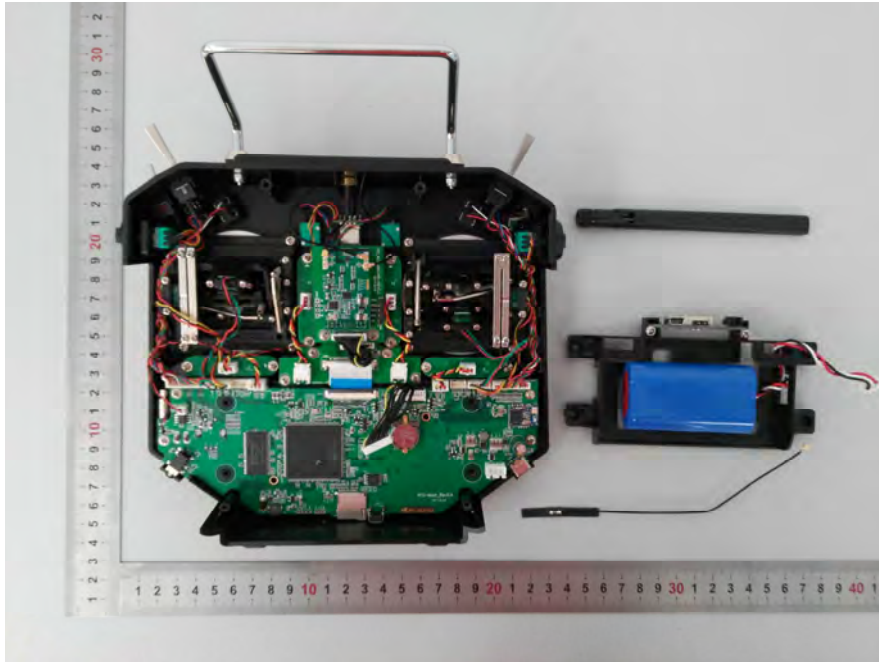
EUT – SRD Antenna Connector View
