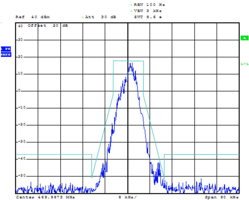
12.5 kHz Channel Spacing, 469.9875 MHz, 4FSK Modulation Only
