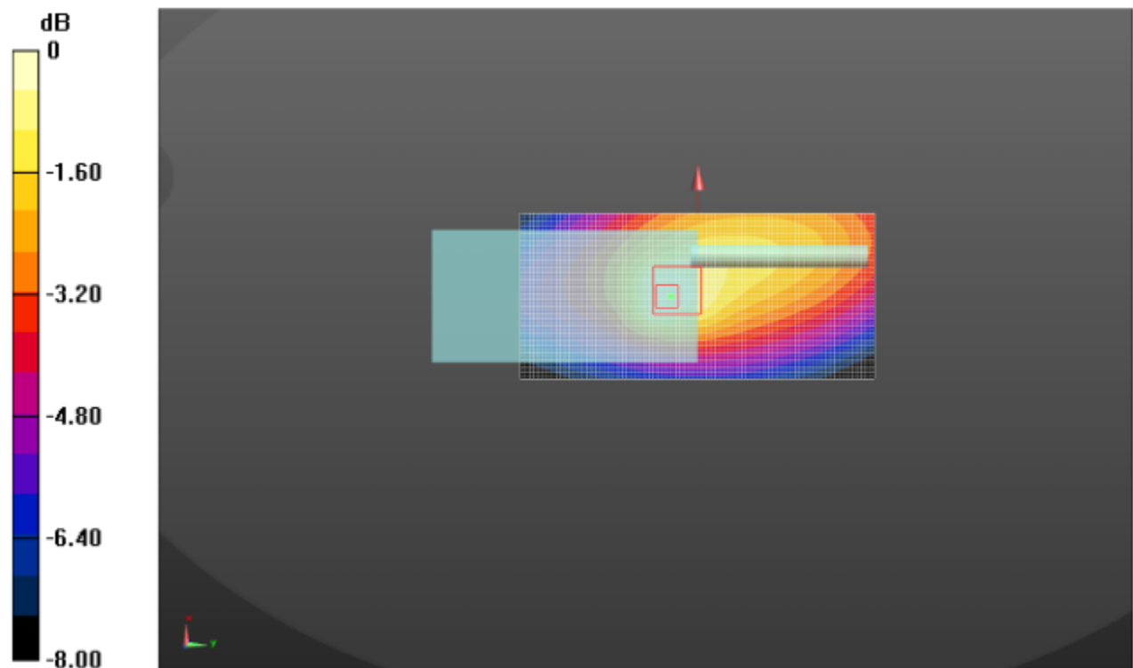
Plot 2: Body-worn for Digital Modulation at 12.5KHz Channel Separation With A1, B1,BC1,S1 and D1; Front towards Ground 469.9875 MHz
