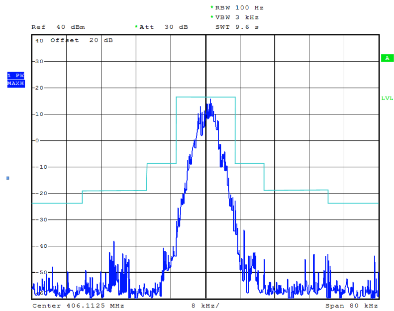
12.5 kHz Channel Spacing, 406.1125 MHz, 4FSK Modulation Only
