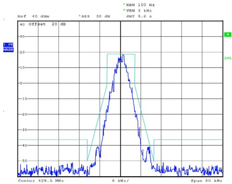
12.5 kHz Channel Spacing, 429.5000 MHz, 4FSK Modulation Only
