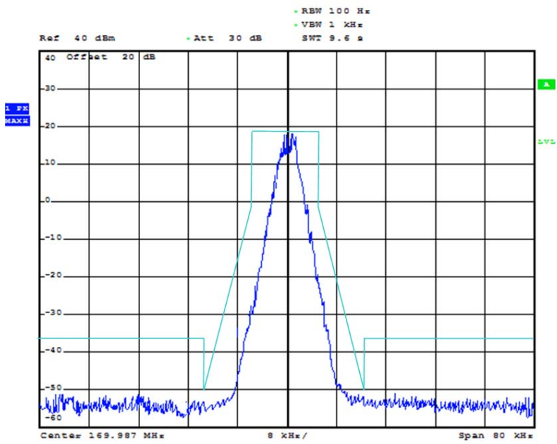
12.5 kHz Channel Spacing, 169.9870 MHz, 4FSK Modulation Only
