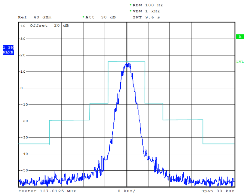
12.5 kHz Channel Spacing, 137.0125 MHz, 4FSK Modulation Only
