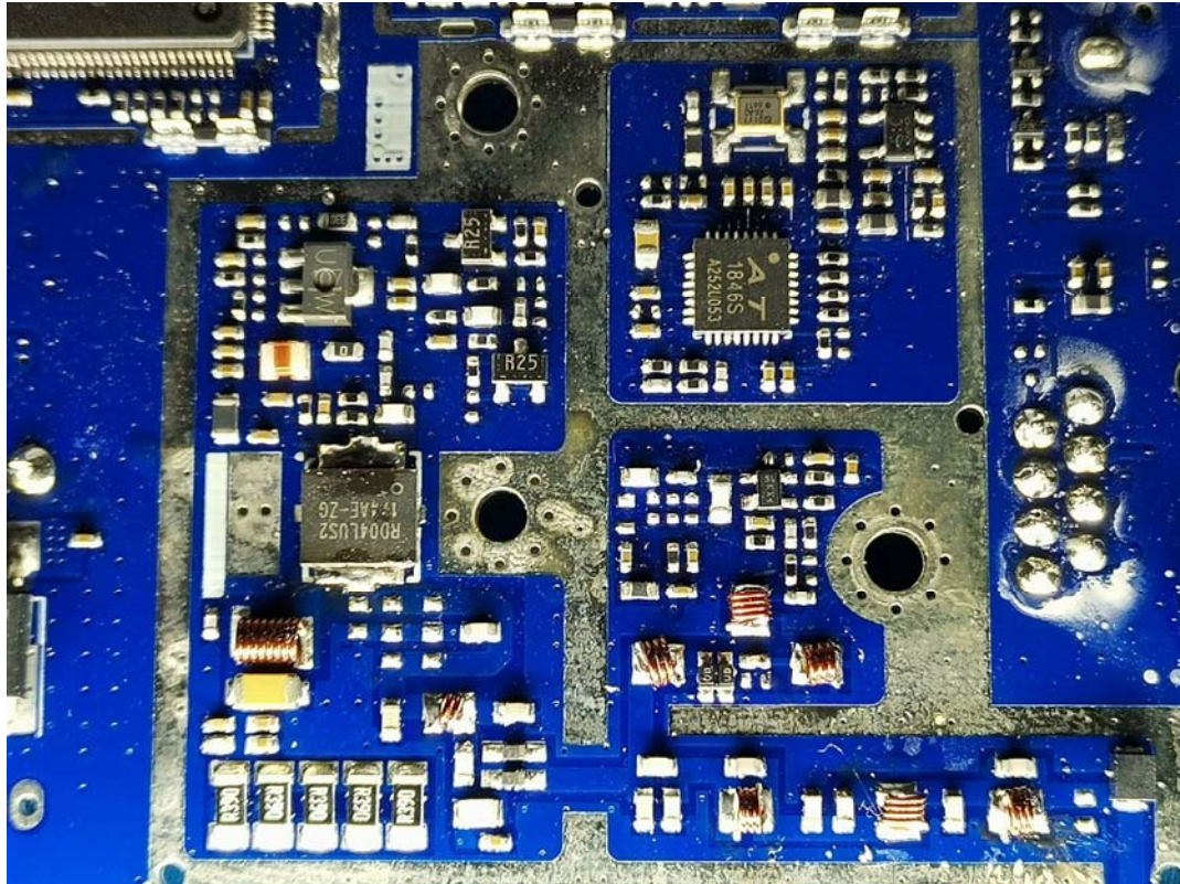
RF Chip
