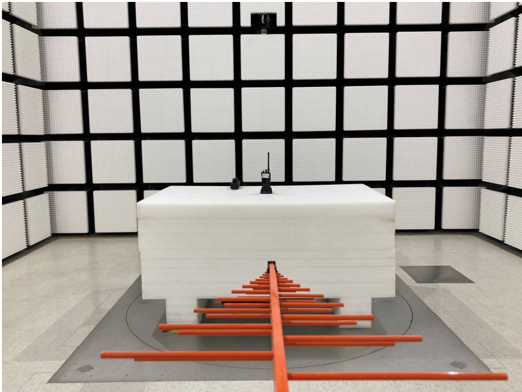
Radiated Emission Below 1GHz View-Model: RDR4250V
