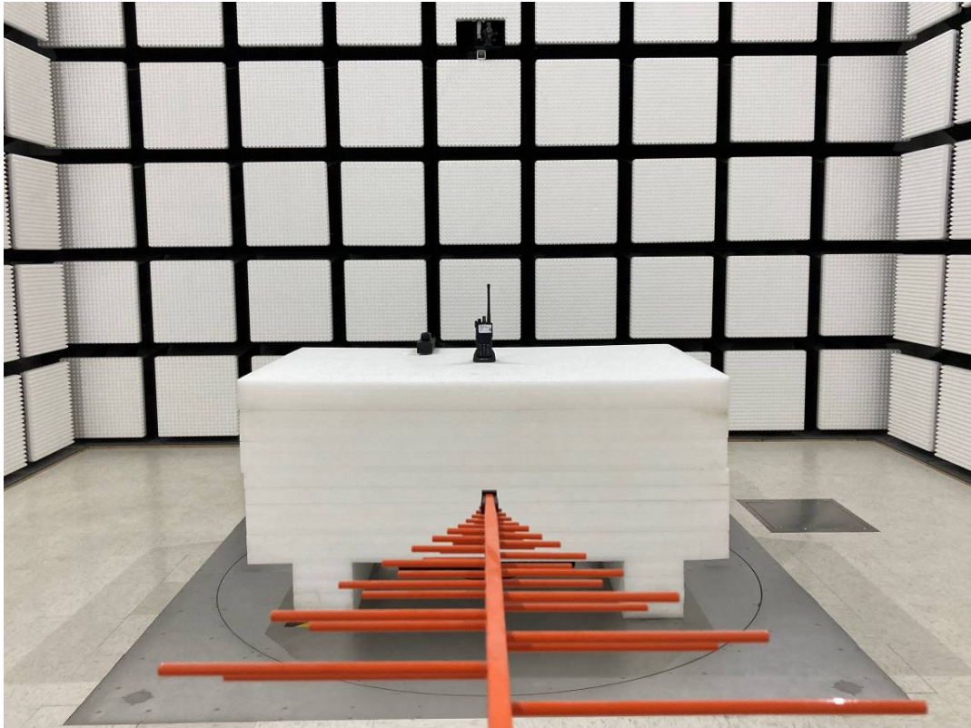
Radiated Emission Above 1GHz View-Model: RDR4280V
