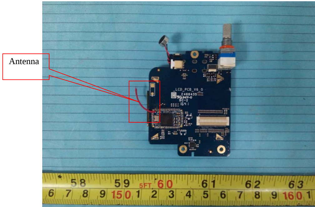
EUT – Main Board 2 Top View (Handset)
