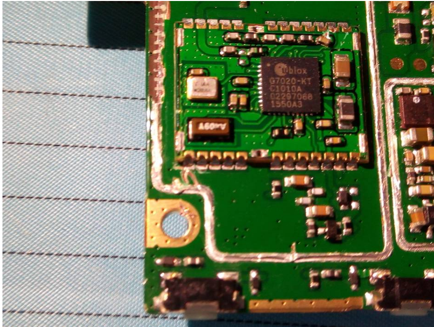
EUT – IC 1 View (Handset)
