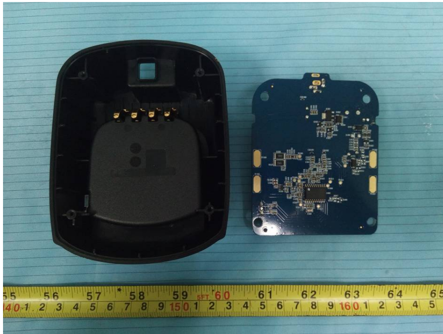
EUT – Cover off View 2 (Charger)
