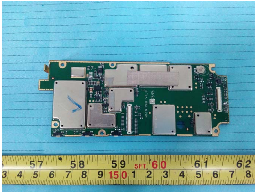
EUT – Main Board 1 Bottom View (Handset)
