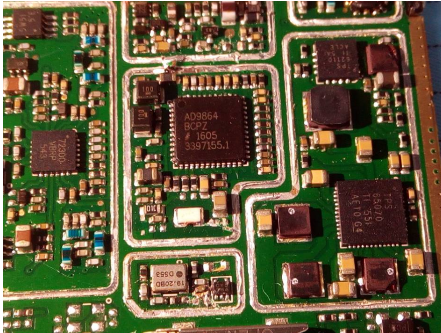
EUT – IC 5 View (Handset)
