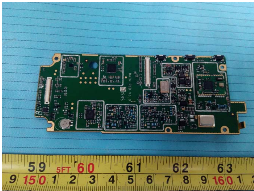
EUT – Main Board 1 Bottom Shielding off View (Handset)
