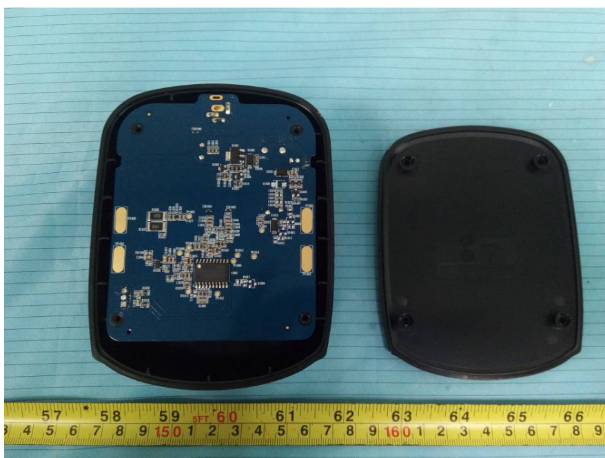
EUT – Cover off View 1 (Charger)
