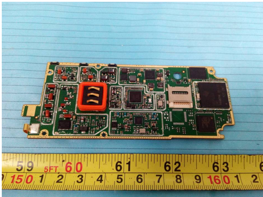
EUT – Main Board 1 Top Shielding off View (Handset)
