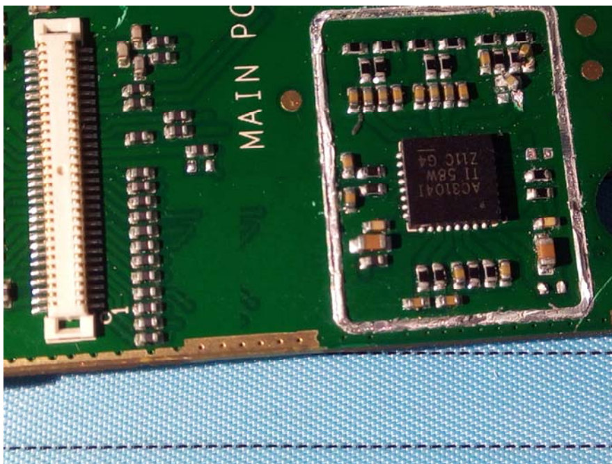
EUT – IC 2 View (Handset)
