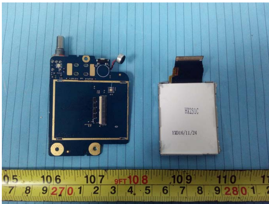
EUT – Cover off View 6 (Handset)
