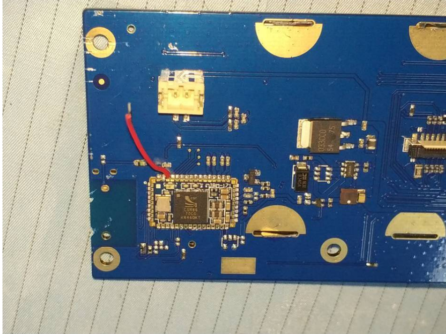
EUT – IC Chip View 5 (Bluetooth)
