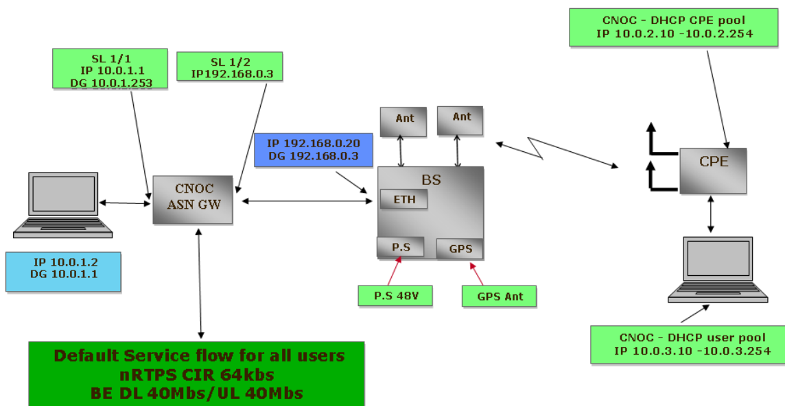
Figure 29 Test Setup Diagram
