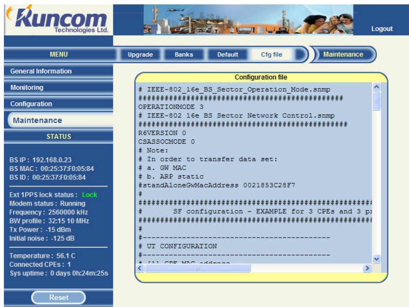
Figure 21 Maintenance – Configuration profile file screen
