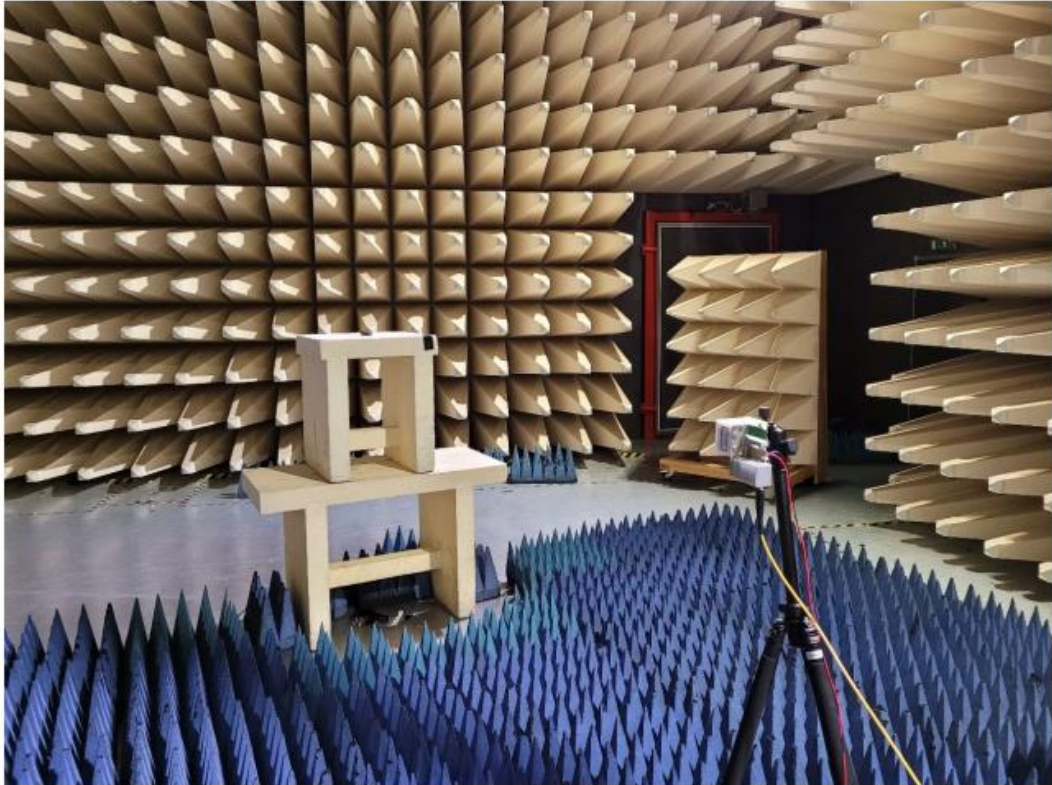
Anechoic Chamber 1: 18 GHz – 26 GHz
