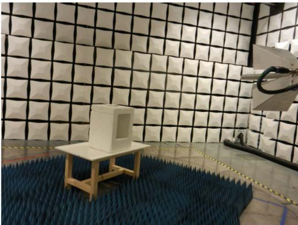
Figure 81 – Test Setup for frequencies >1 GHz
