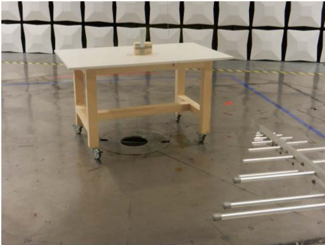
Figure 80 – Test Setup for frequencies 30 MHz – 1 GHz
