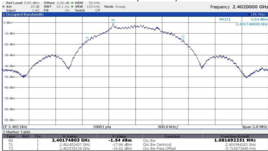
Channel 37 (2402 MHz)
