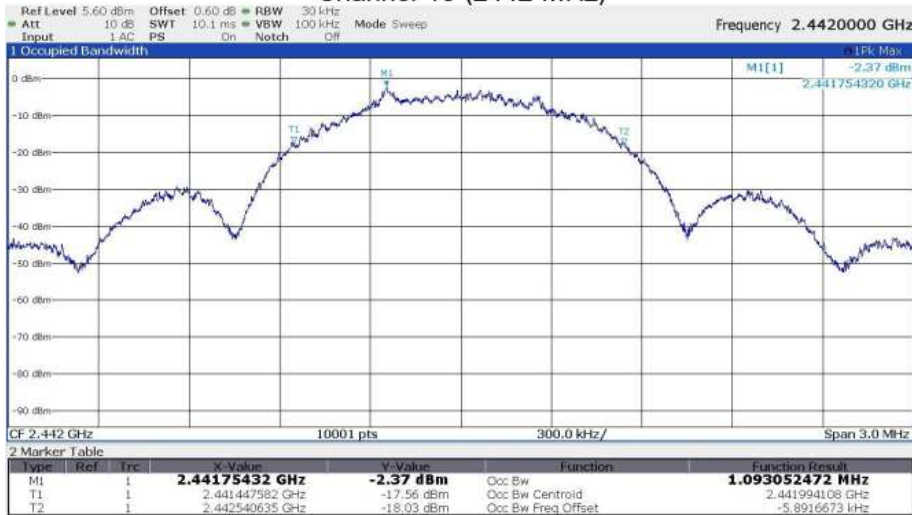
Channel 18 (2442 MHz)
