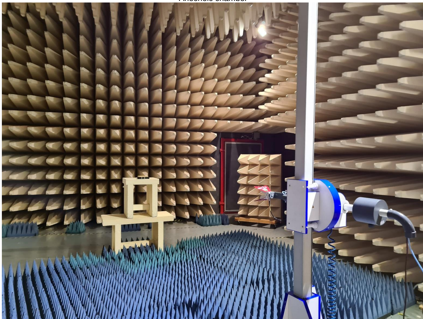
Anechoic chamber
