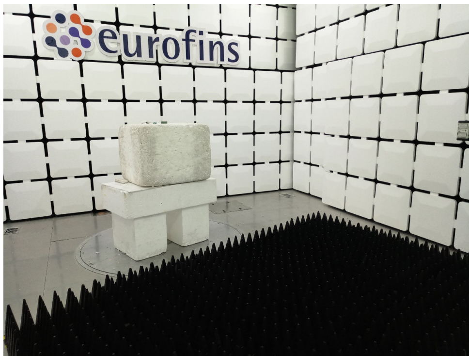
18GHz - 26.5GHz Picture 1: Radiated Spurious Emissions Test setup
