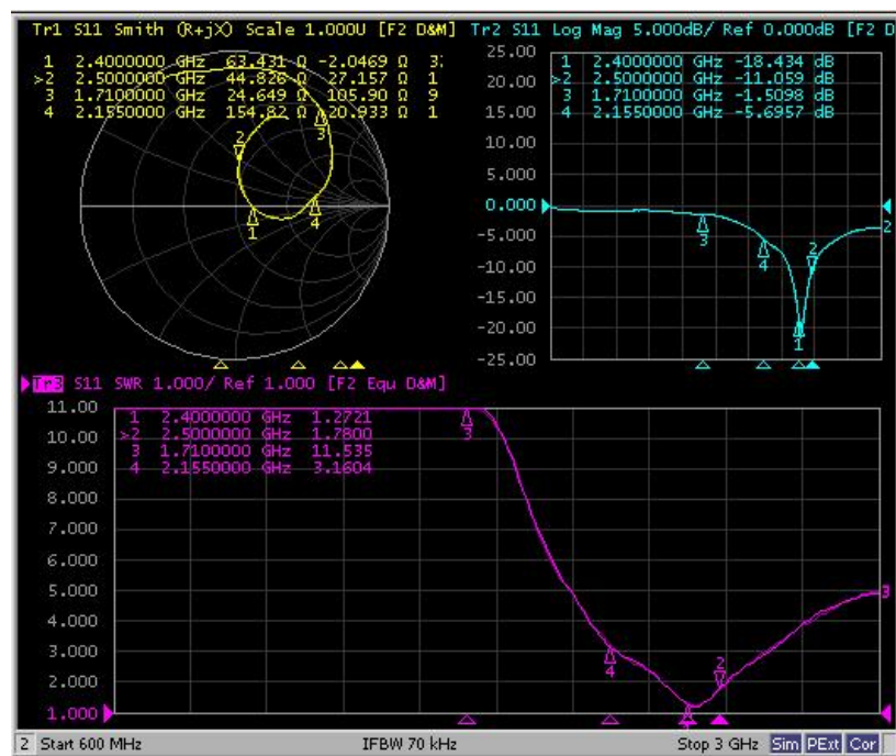
BT Antenna
