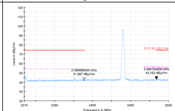
Bandedge:2M Ch19
