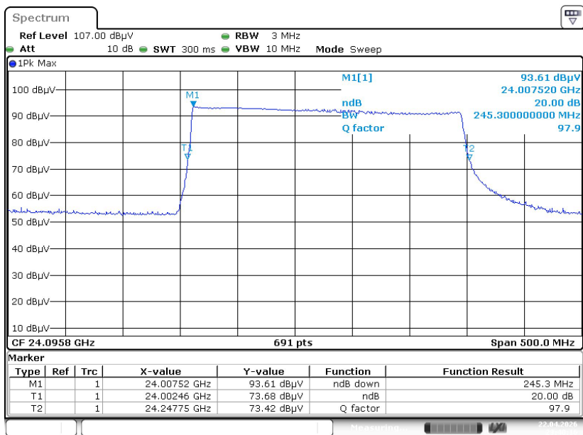
20 dB Bandwidth
