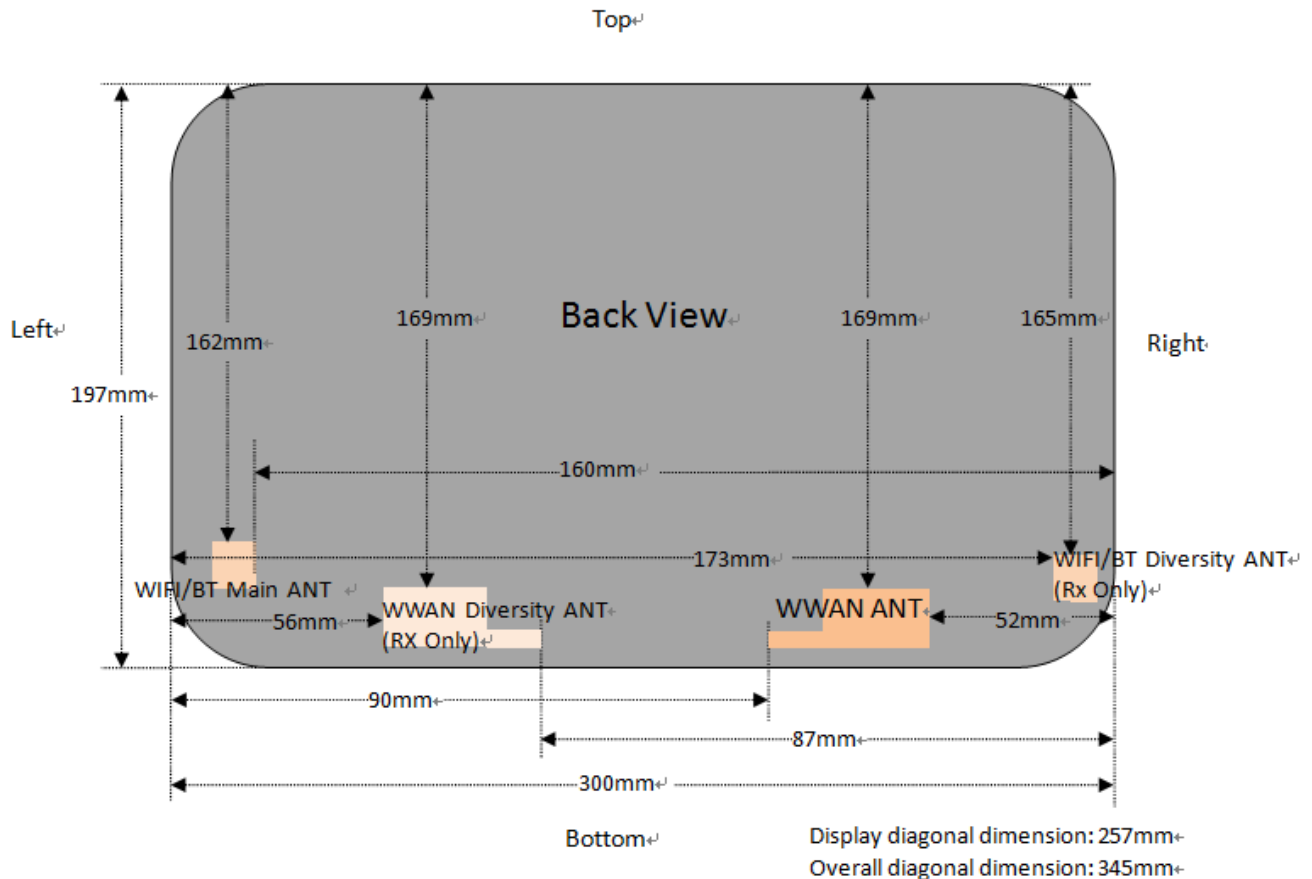
Fig.14.1 EUT Antenna Locations (Back View)
