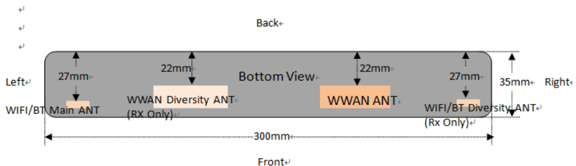
Fig.14.2 EUT Antenna Locations (Bottom View)
