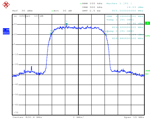
99% Occupy bandwidth
