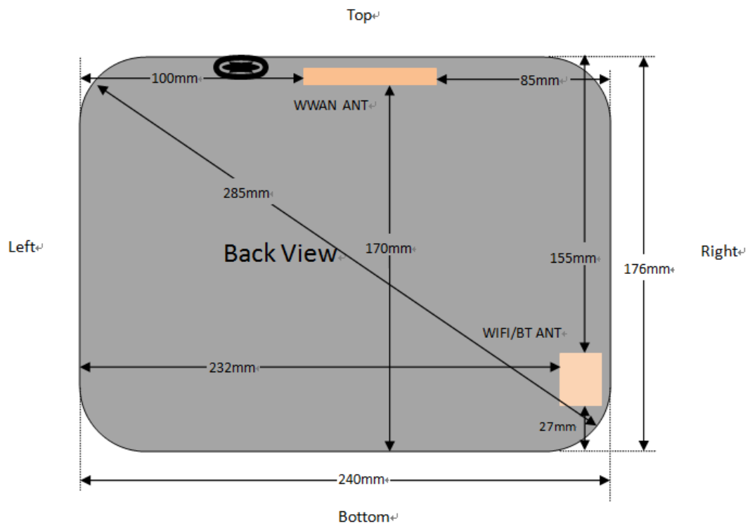
Fig.14.1 EUT Antenna Locations
