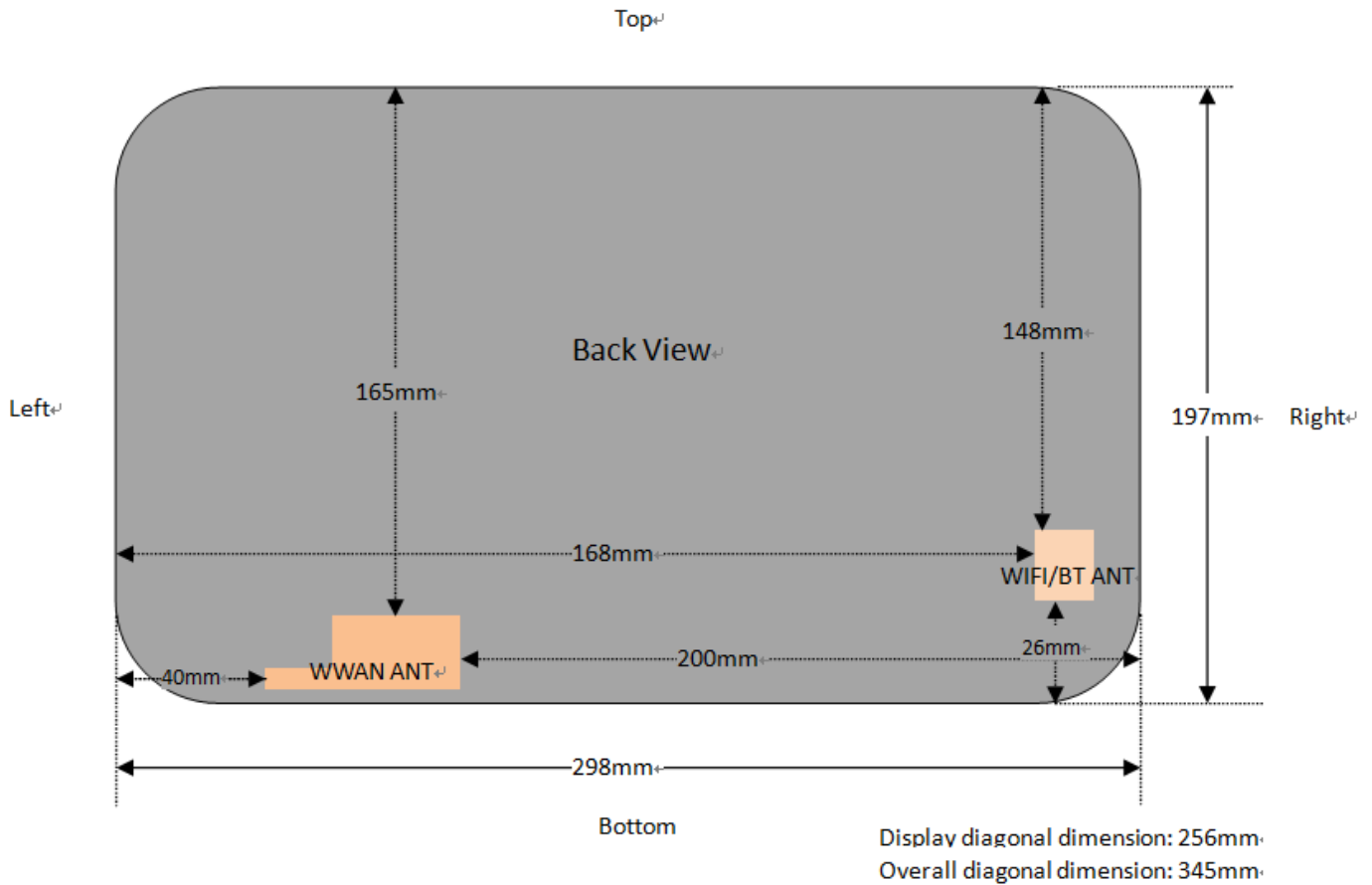
Fig.14.1 EUT Antenna Locations
