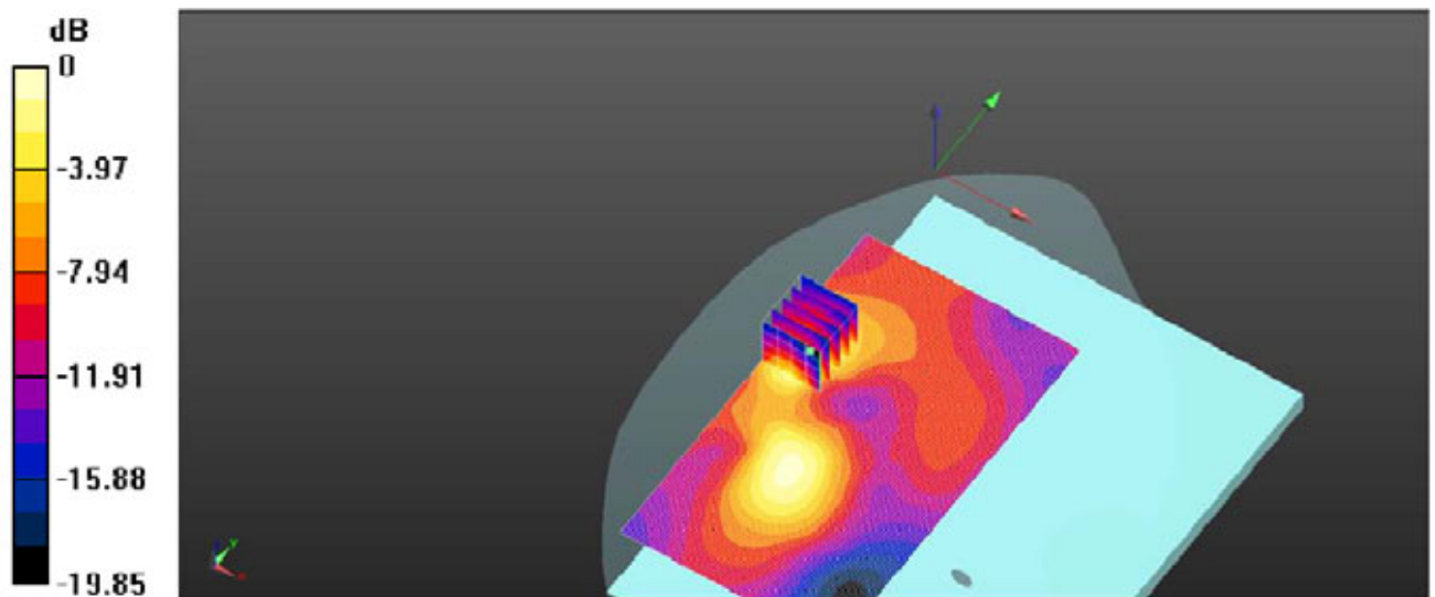
Plot 5: Body Rear Side (GSM850 EGPRS 4TS Middle Channel)
