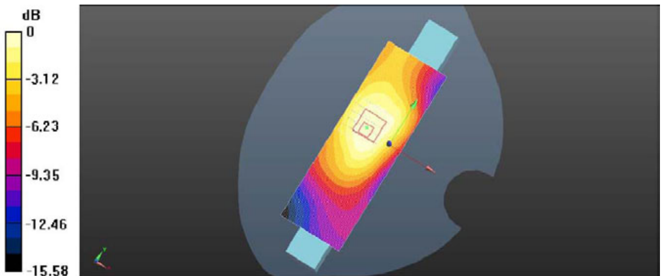
Plot 2: Body Left Side (GSM850 GPRS 4TS Middle Channel)
