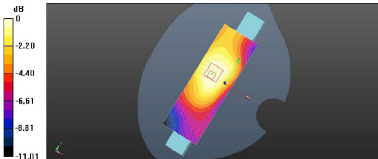
Plot 10: Body Left Side (WCDMA Band II RMC Middle Channel)
