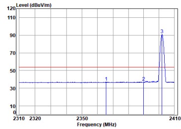
BLE_TX_CH_00_Vertical-AVG
