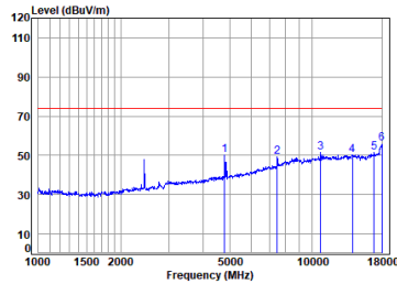
BLE_TX_CH_19_Vertical-Peak
