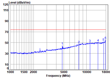
BLE_TX_CH_19_Horizontal-Peak
